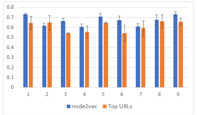
Fig. 3. Imbalanced Classification comparing baseline (top URLs) and node2vec on a 10-fold cross-validation
